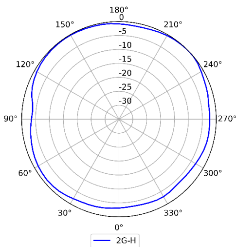
2.4GHz (Horizontal)
